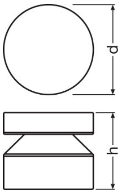
LED SURFACE POLE 6 W 3000 K SST
